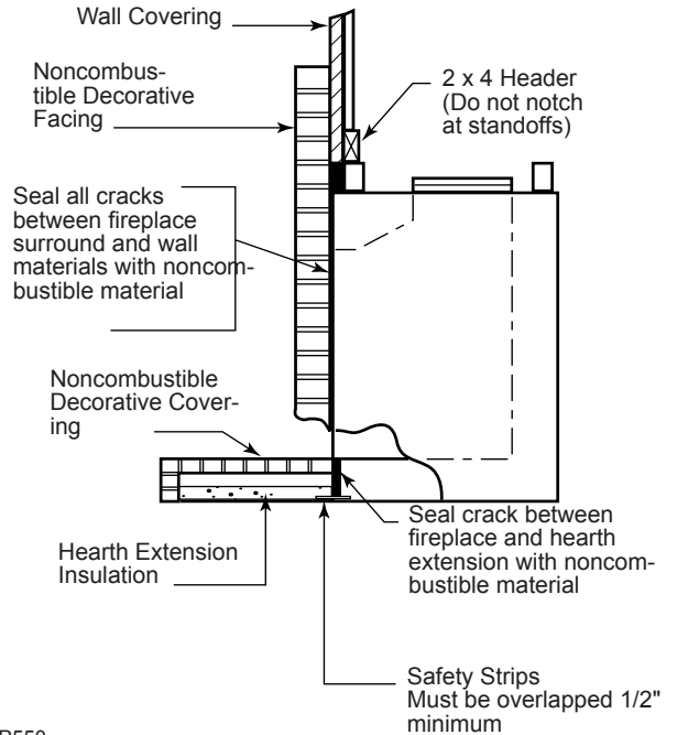
Fig. 25 Sealing gaps.
