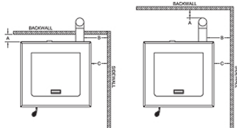
SIDEWALL CLEARANCES PARALLEL INSTALATION
