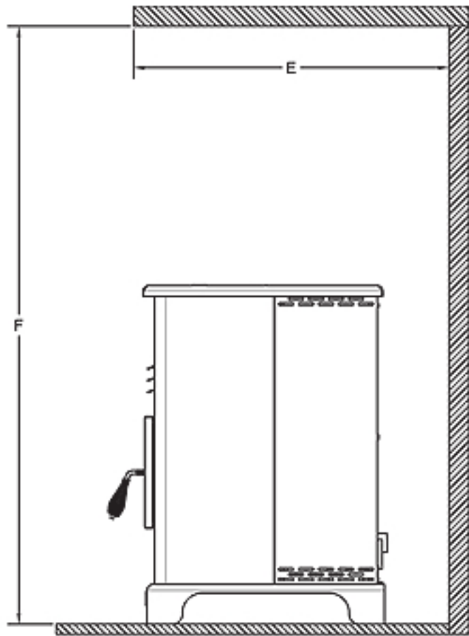
ALCOVE CLEARANCES
