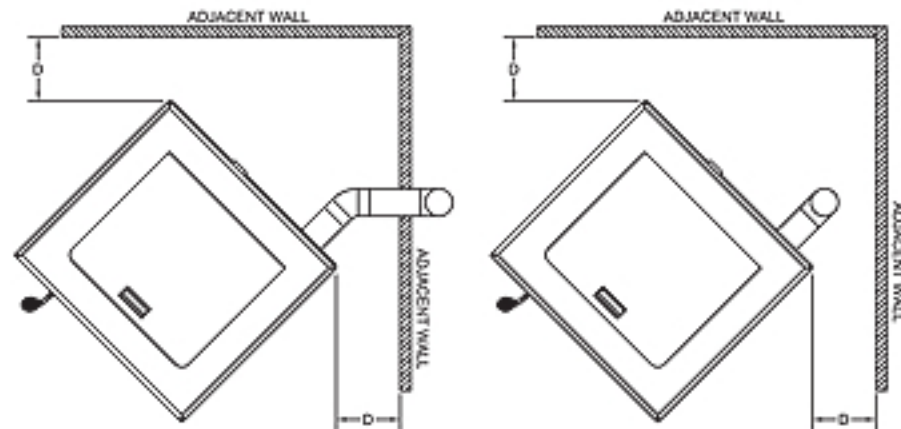
SIDEWALL CLEARANCES CORNER INSTALATION
